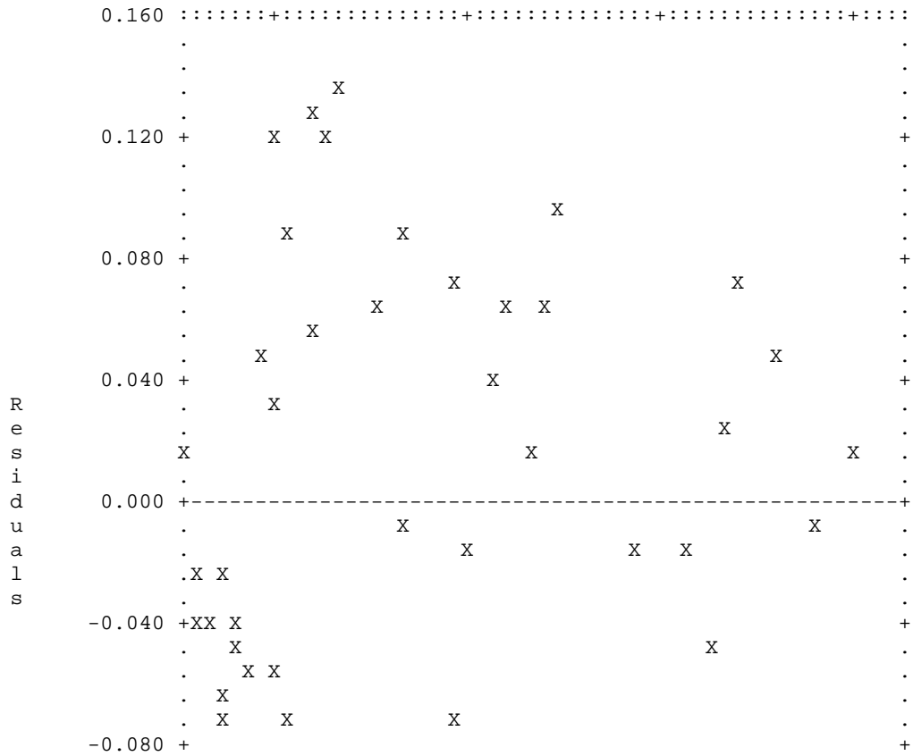
Residual Plot
