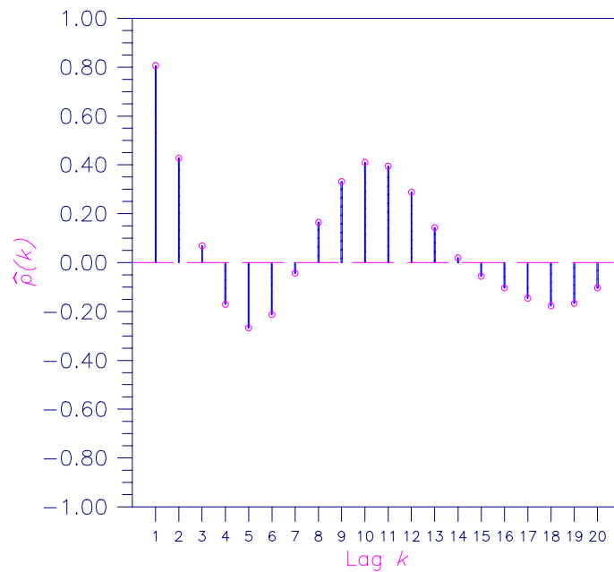
Figure 8-2-Sample Autocorrelation Function
