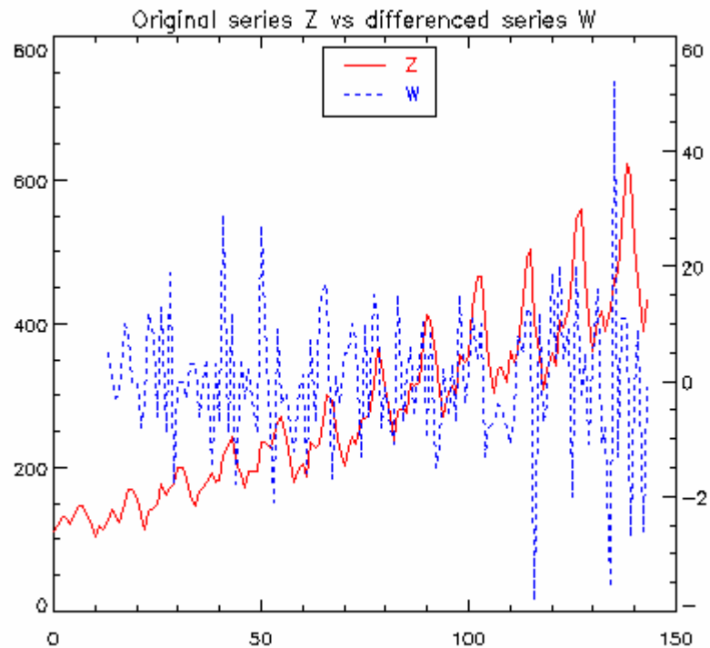
Figure 8-1-Differenced Series
